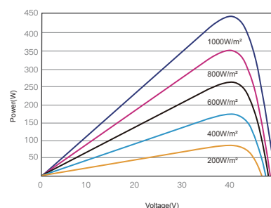
P-V CURVES OF PV MODULE(445W)
