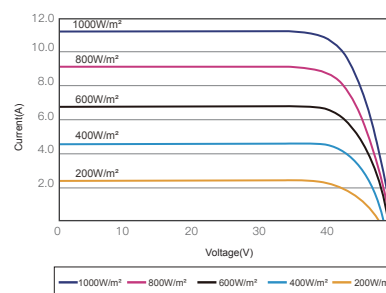
I-V CURVES OF PV MODULE(445W)
