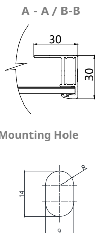
Frame Cross Section
