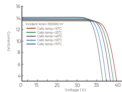
Current-Voltage Curve
