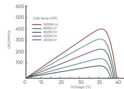
Power-Voltage Curve
