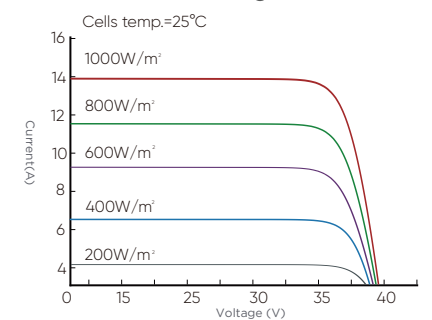
Current-Voltage Curve
