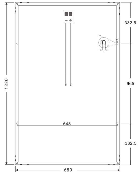
Mechanical Diagrams
