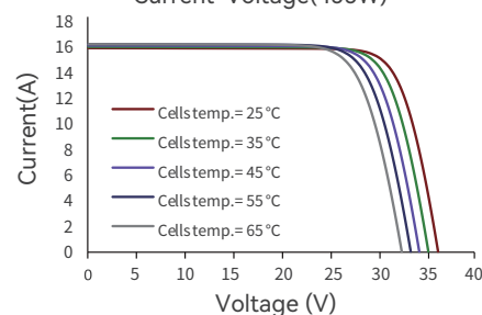
Current-Voltage(455W)
