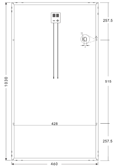
Mechanical Diagrams
