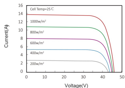
Current-Voltage Curve (JFS2-132-18X)
