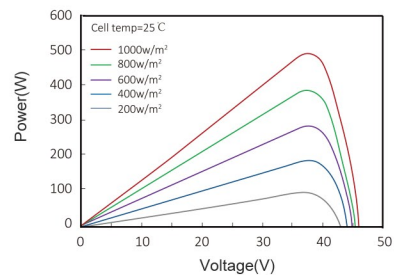
Power-Voltage Curve (JFS2-132-18X)
