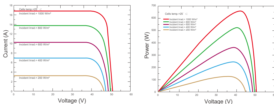
Current-Voltage & Power-Voltage Curves (RMHHB66-700S3)
